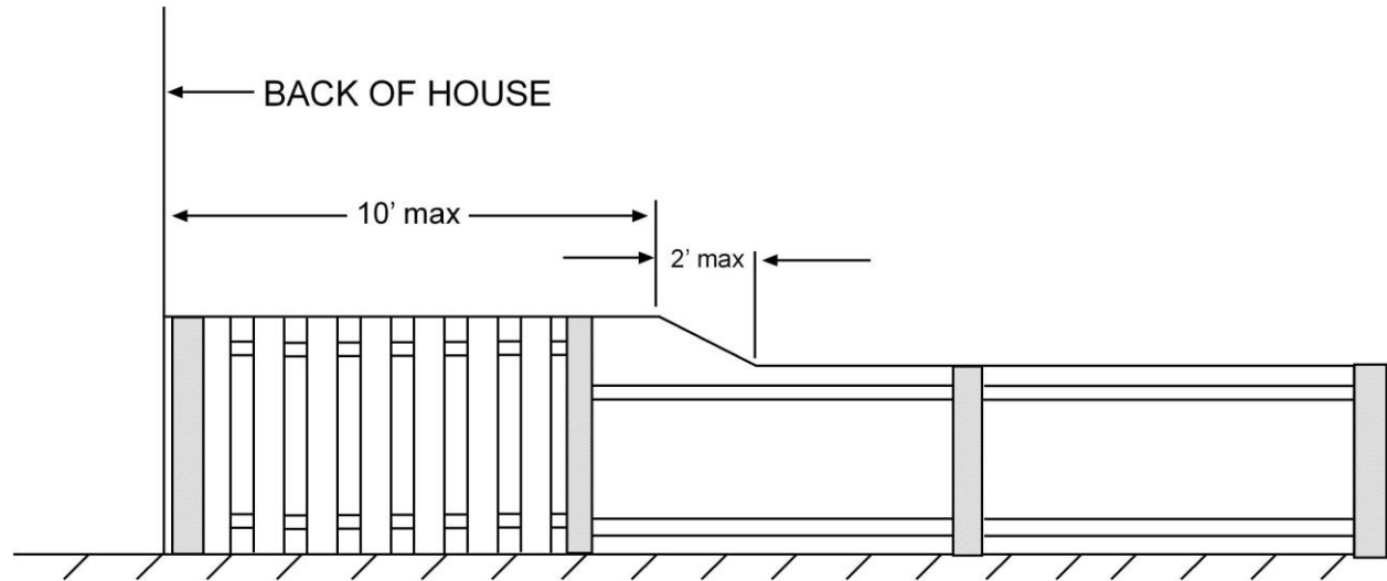
SIDE VIEW
